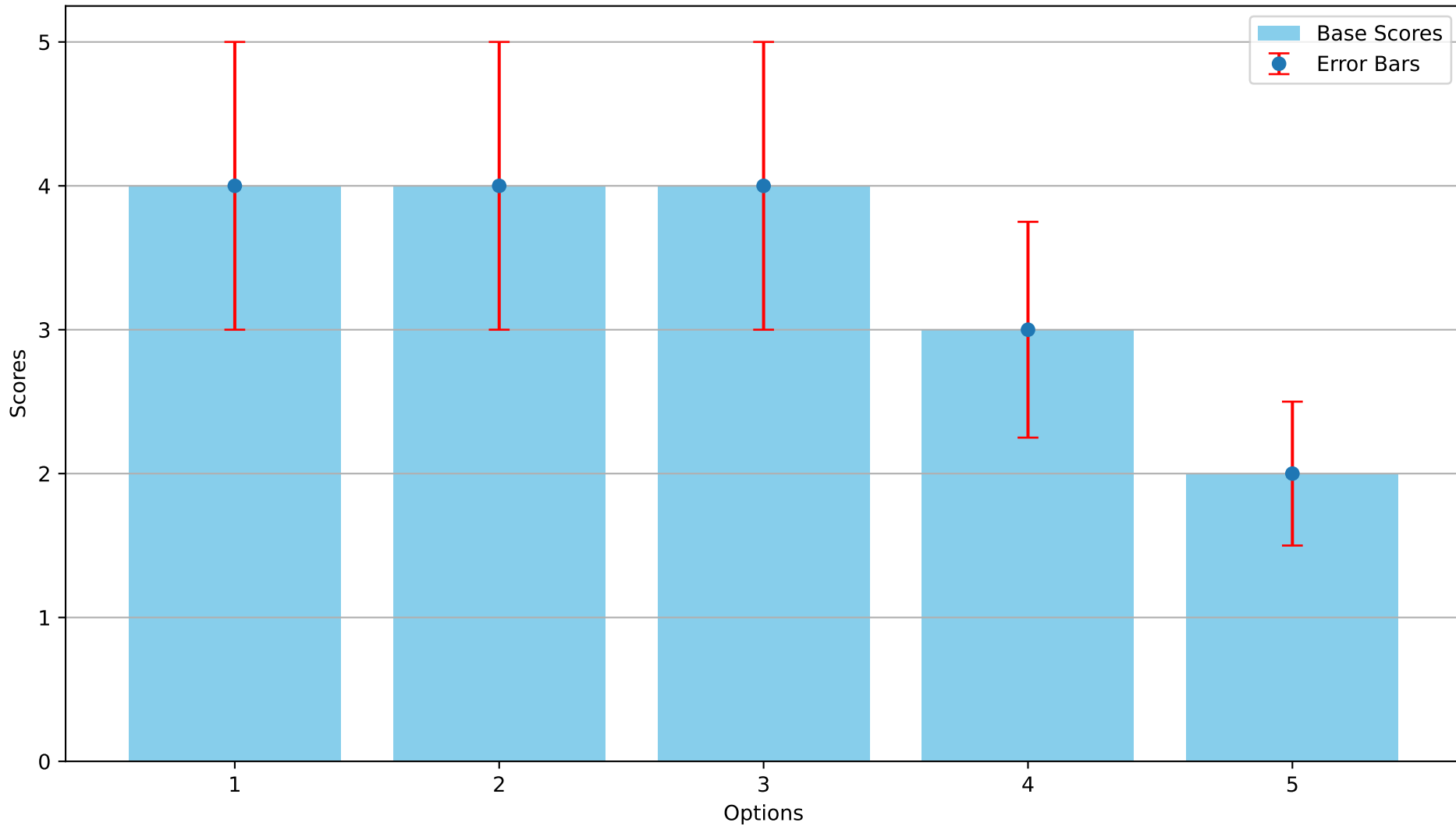
Combined Result Sensitivity Analysis for Operational
